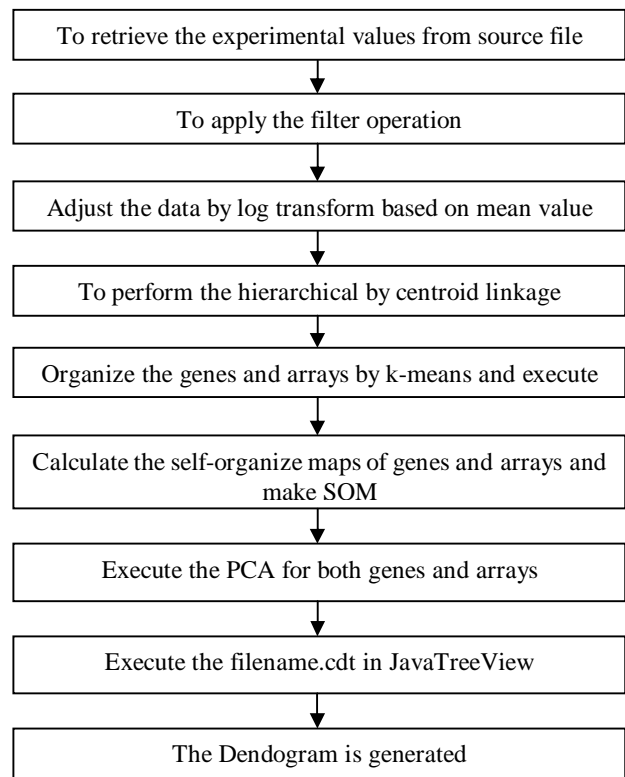
Fig 2: The execution of clustering process
