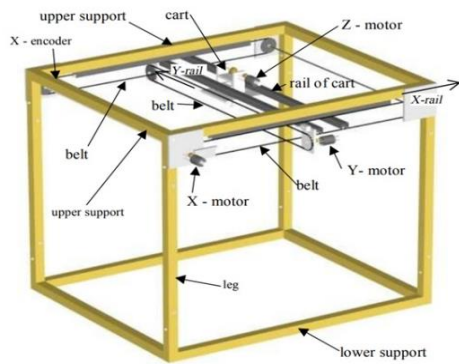
Figure 1: the 3D Crane model with actuators and sensors.
