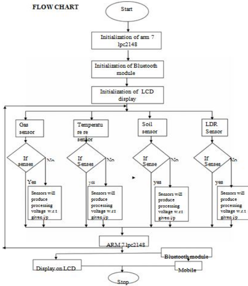
Fig: 1 Design and Implementation
