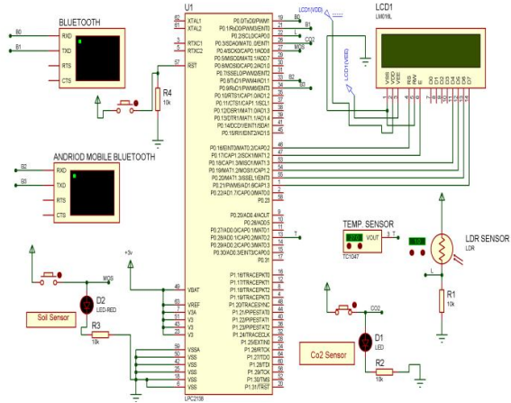
Fig: 1.3 Application and working Diagram of Wireless sensors based data acquisition system using smart mobile
