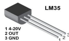
Fig: 2 Temperature Sensors
