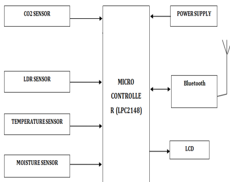
Fig: 1.2 Hardware Block Diagram
