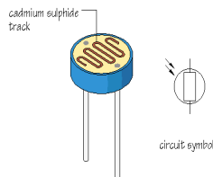
Fig: 2.1 Light Dependent Resistors (LDR)
