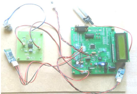
Fig: 3 System developed interface wireless sensors with ARM7 and interface Wireless Bluetooth
